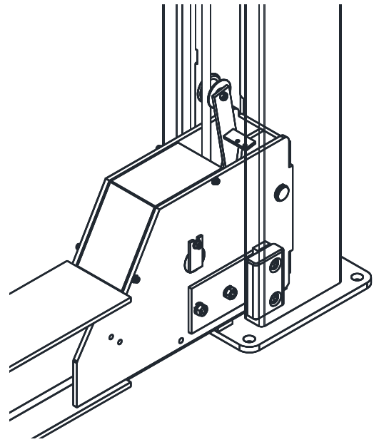
Fig 8 – Slide Block Installation
