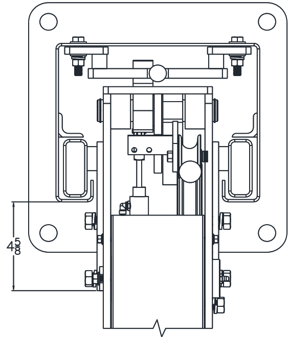
Fig 9 – Column Positioning
