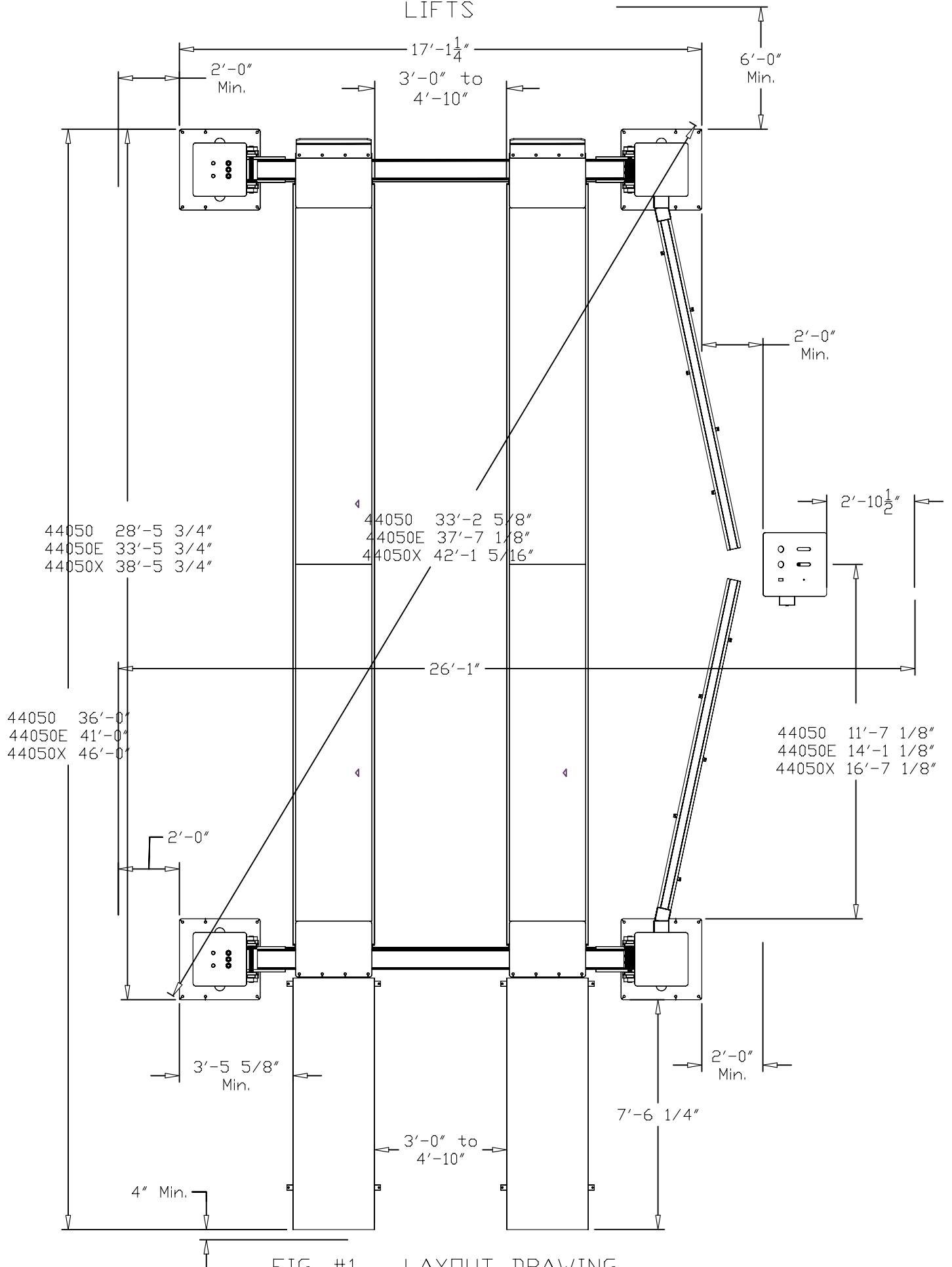
FIG. #1 LAYOUT DRAWING 44050, 44050E & 44050X LIFT
