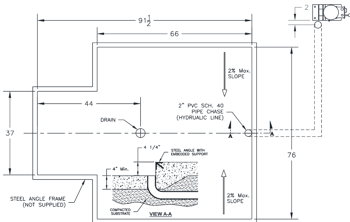
Fig. 1B - General Flush Mount Layout
