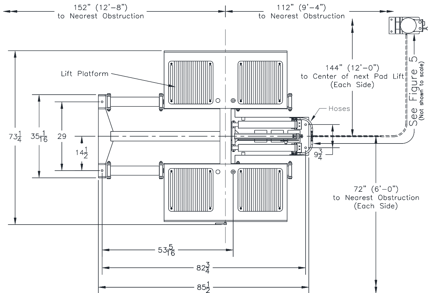
Fig. 1B - General Flush Mount Layout
