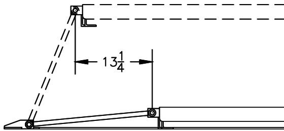
Fig. 3 Rearward Movement
