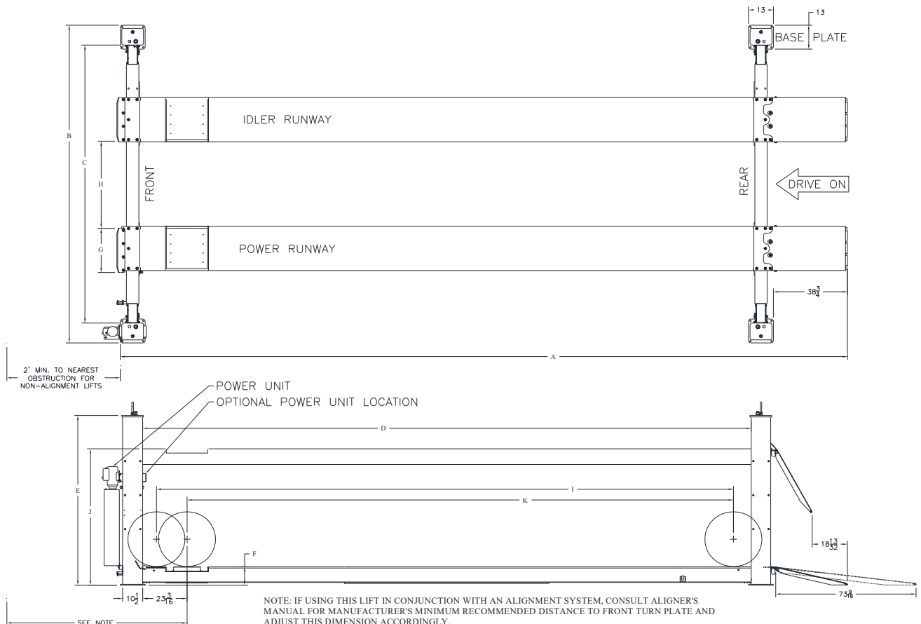
Fig 1 – General Specifications and Service Bay Layout
