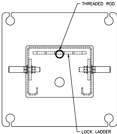
Fig 14 – Locking Ladder Orientation
