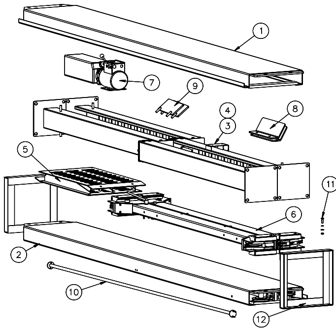
Fig 3 – Package Components
