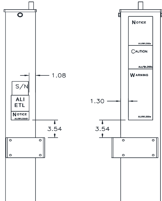
Fig 23 – Power Column Decal Location
