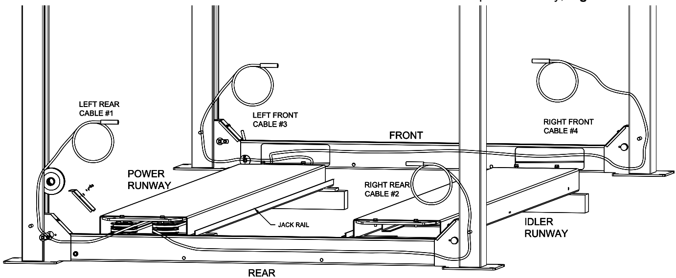
Fig 7 – Runway Layout
