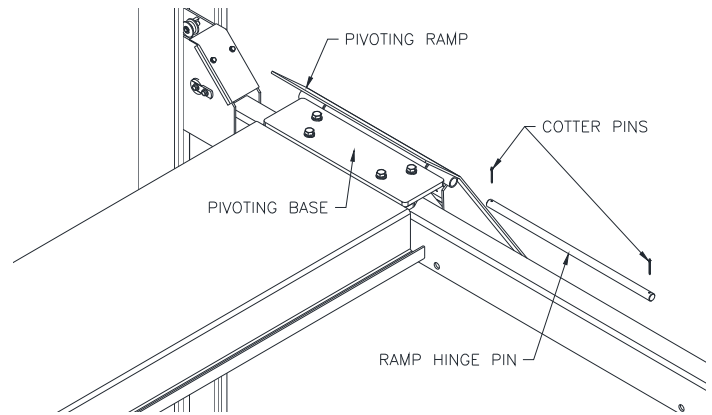
Fig 33 – Ramp Installation
