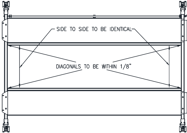
Fig 13 – Final Runway Positioning
