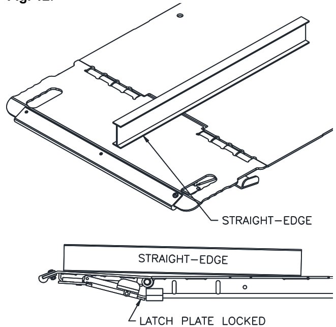
Fig. 12 LEVELING THE RAMPS WITH A STRAIGHT- EDGE
