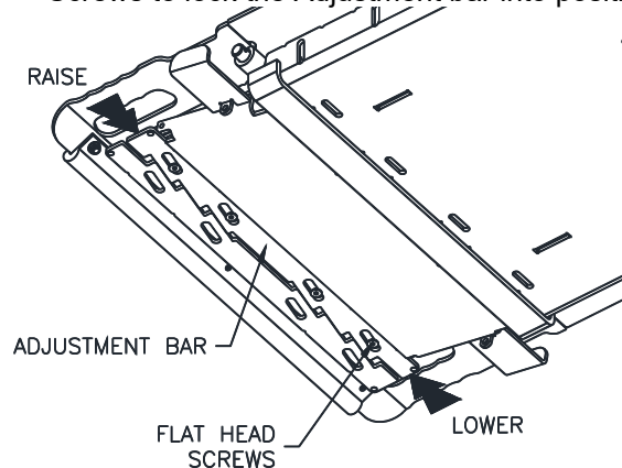
Fig. 13 MOVING THE SAW-TOOTHED ADJUSTMENT BAR
