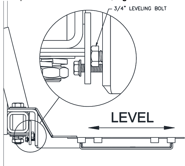
Fig. 4 LEVELING THE PAD ADAPTERS
