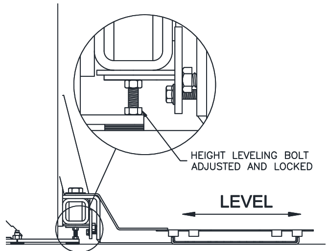
Fig. 9 SETTING THE HEIGHT LEVELING SCREWS
