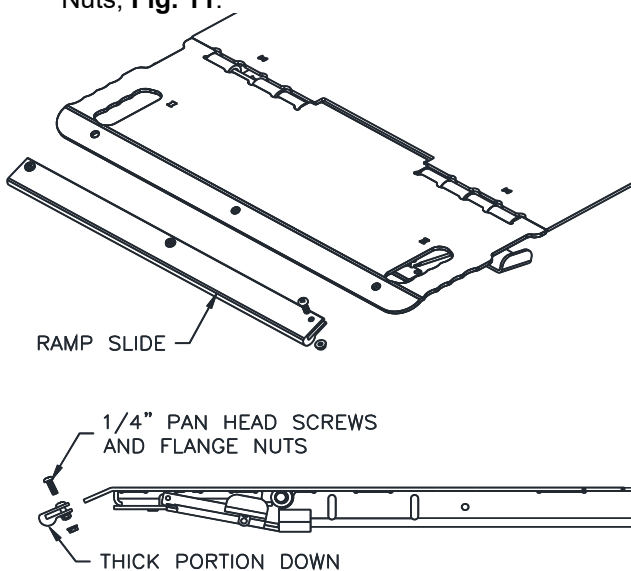
Fig. 11 INSTALLING THE RAMP SIDES
