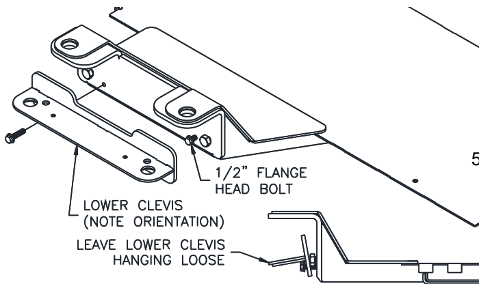
Fig. 2 ATTACHING LOWER CLEVIS PLATE
